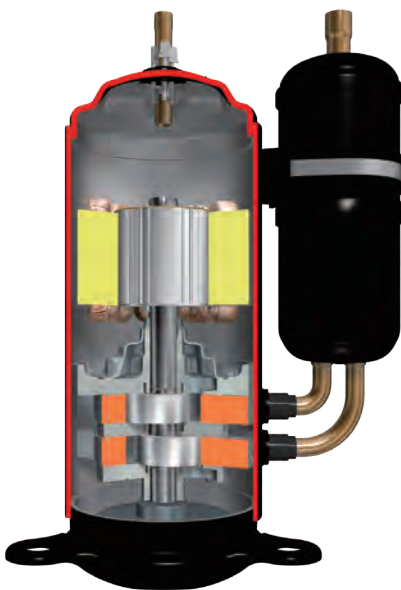
2 Cylinder rotary compressor NEW High power series
